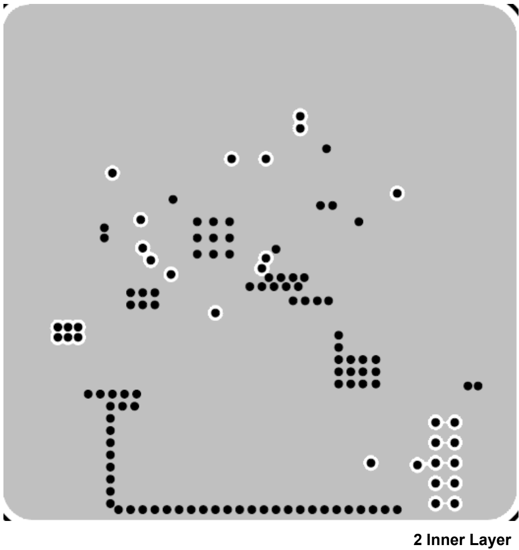
Figure 25. Layout Guide (2 Inner Layer)
