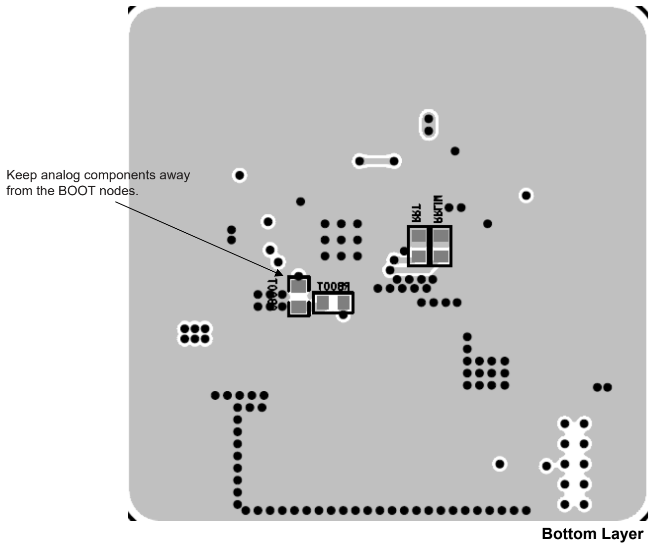
Figure 27. Layout Guide (Bottom Layer)
