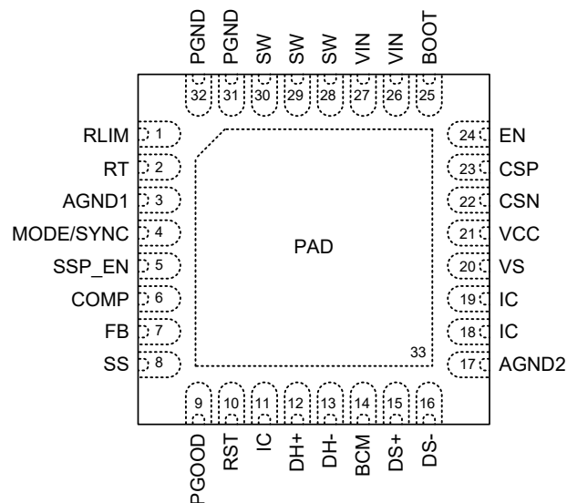
WETD-VQFN-32L 5x5
