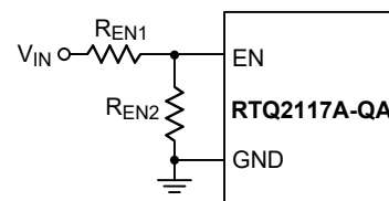
Figure 20. Resistive Divider for Undervoltage-Lockout Threshold Setting
