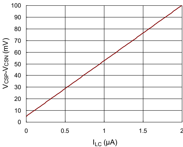
Figure 17. I_{LC} vs. V_{CSP} - V_{CSN}
