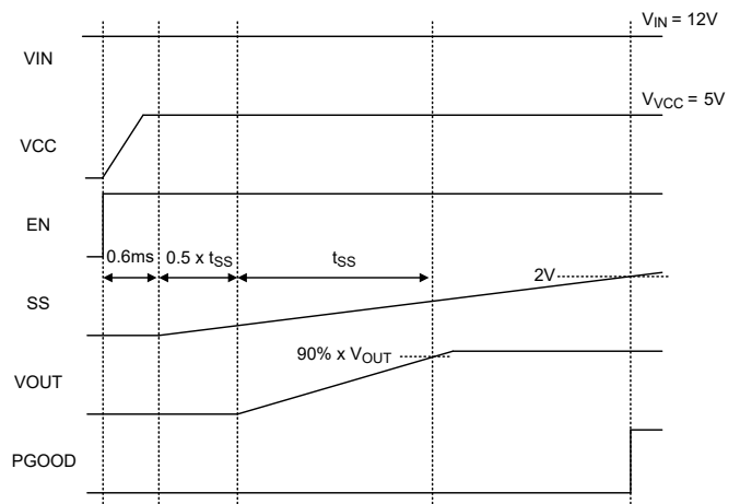
Figure 1. Start-Up Sequence
