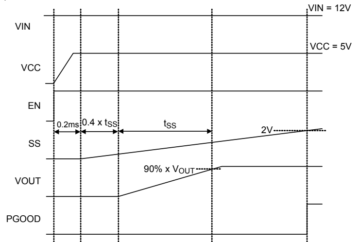
Figure 1. Start-Up Sequence
