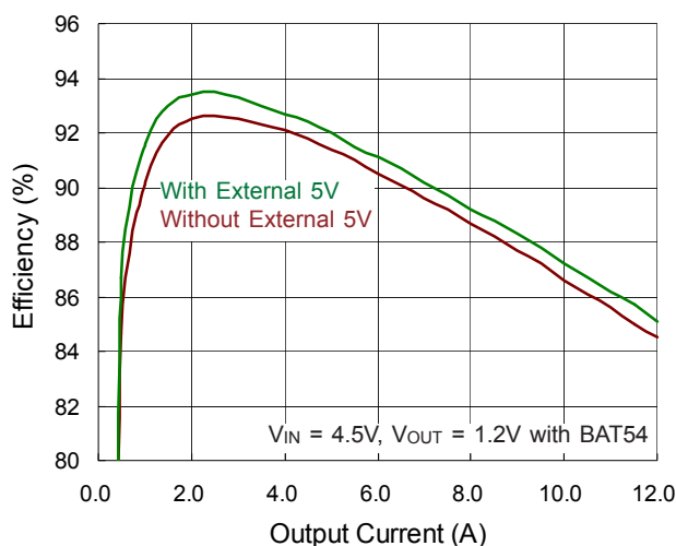
Figure 8. Efficiency Comparison with/without external 5V supply
