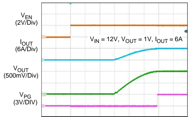
Time (10ms/Div)
