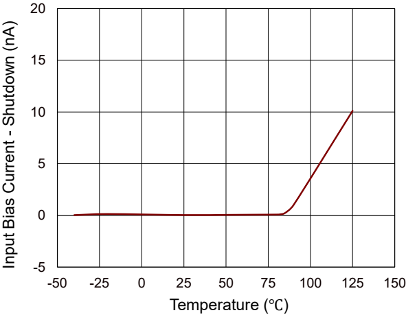
Input Bias Current vs. Temperature (Shutdown)
