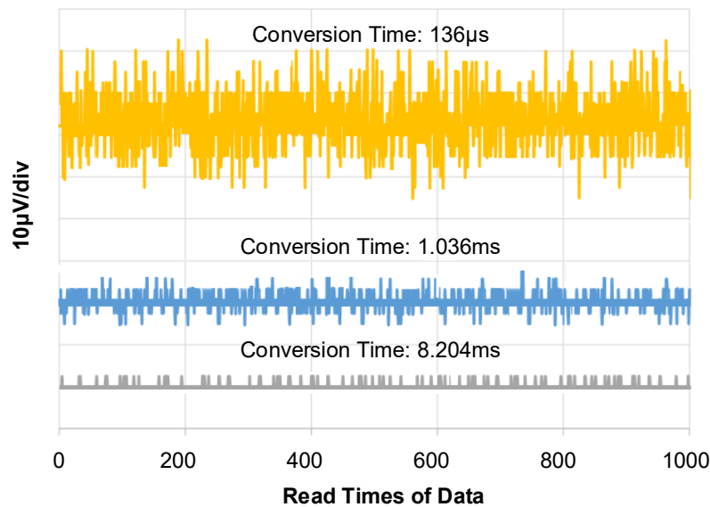
Figure 2. Noise vs. Conversion Time
