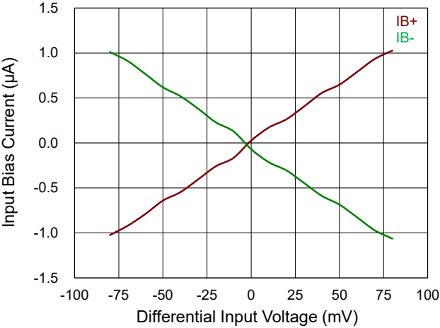
Input Bias Current vs. Differential Voltage
