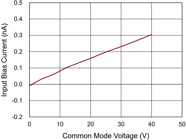
Input Bias Current vs. Common-Mode Voltage (IB+, IB-)
