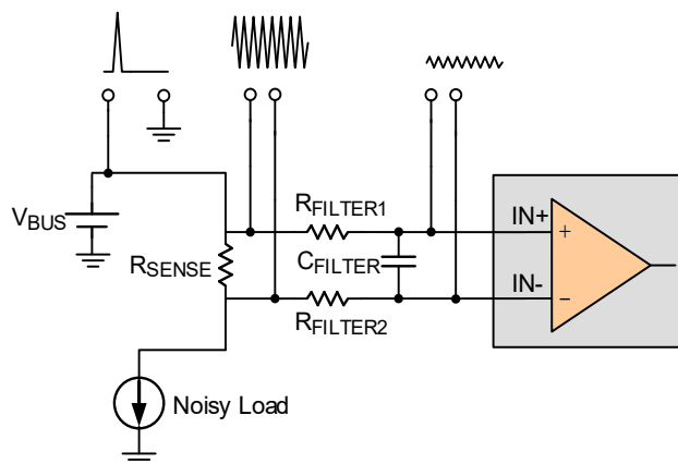
Figure 6. Input Filtering
