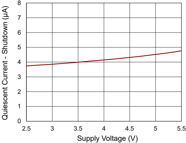
Quiescent Current - Shutdown vs. Supply Voltage
