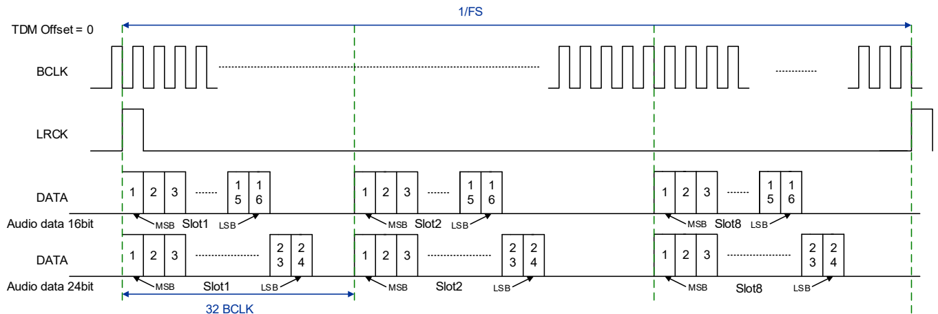
Figure 8. TDM (Offset = 0)
