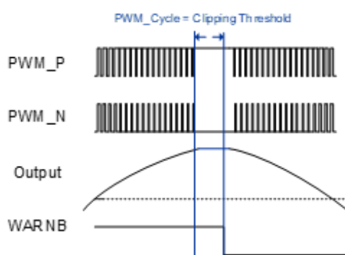
Figure 17. Clip Detection
