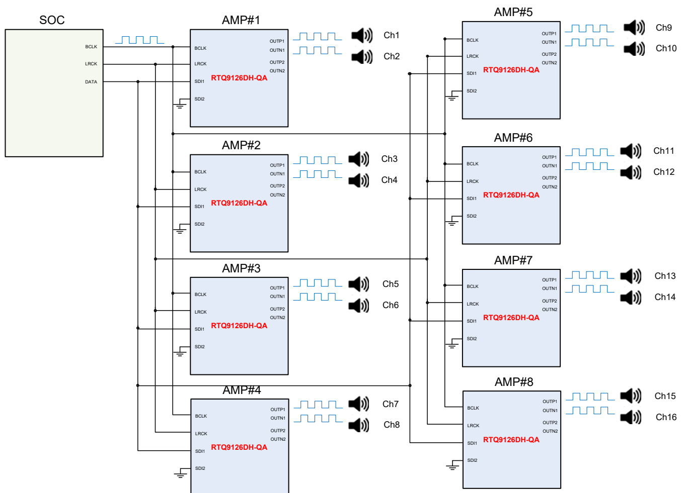
Figure 9. TDM16
