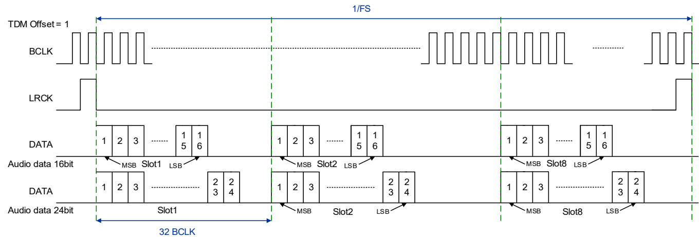
Figure 7. TDM (Offset = 1)
