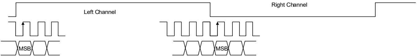
Figure 5. Left-Justified
