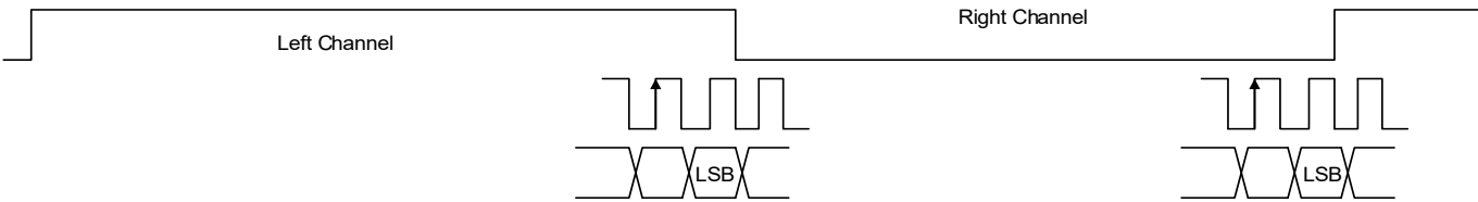
Figure 6. Right-Justified
