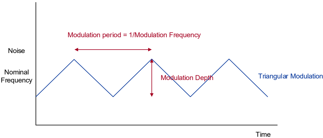
Figure 15. Spread-Spectrum Algorithm
