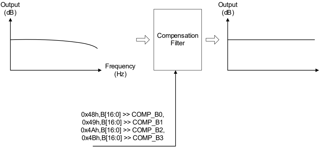
Figure 11. Compensation Filter
