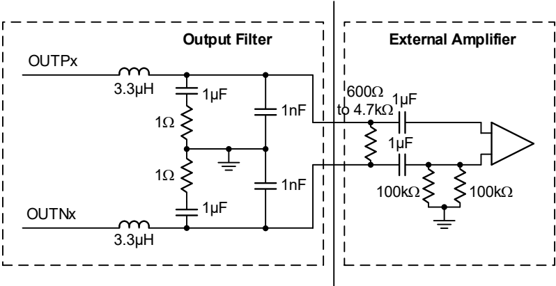
Figure 18. Output Filter
