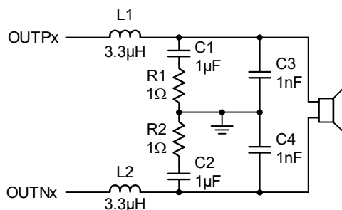
Figure 19. Output Filter
