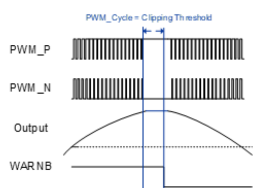
Figure 18. Clip Detection
