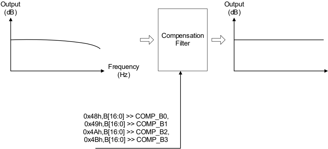
Figure 11. Compensation Filter
