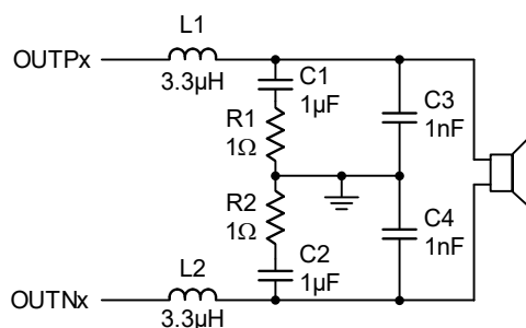
Figure 20. Output Filter
