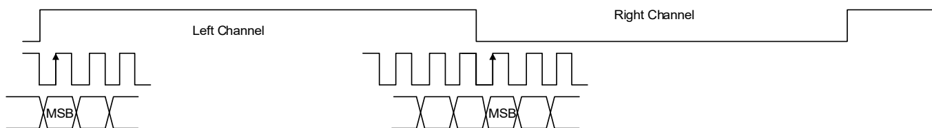
Figure 5. Left-Justified
