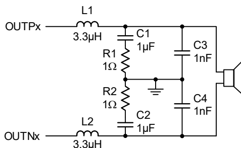
Figure 19. Output Filter
