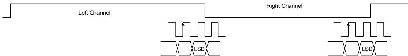
Figure 6. Right-Justified
