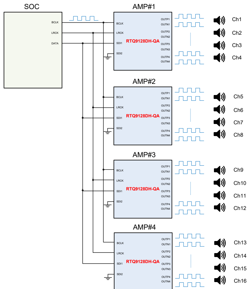
Figure 9. TDM16
