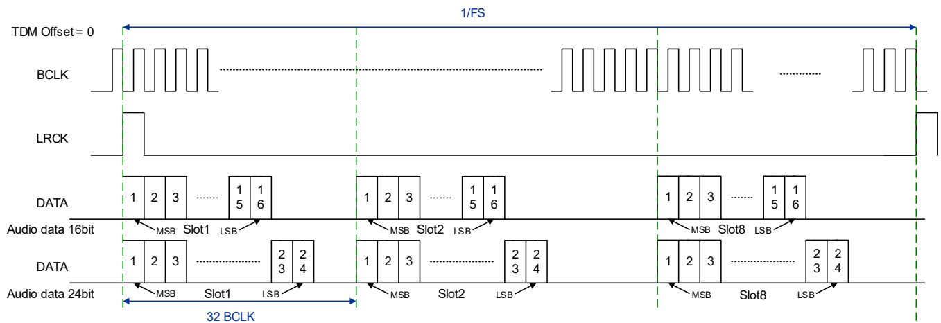
Figure 8. TDM (Offset = 0)
