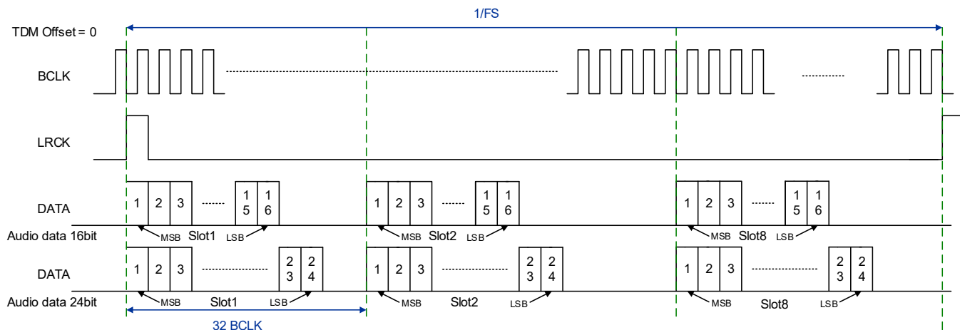
Figure 8. TDM (Offset = 0)
