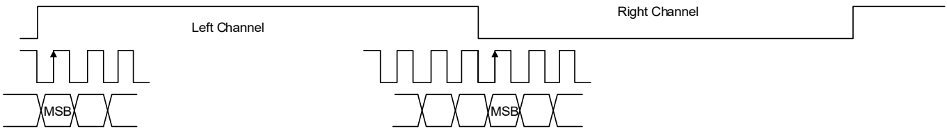
Figure 5. Left-Justified
