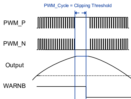
Figure 18. Clip Detection
