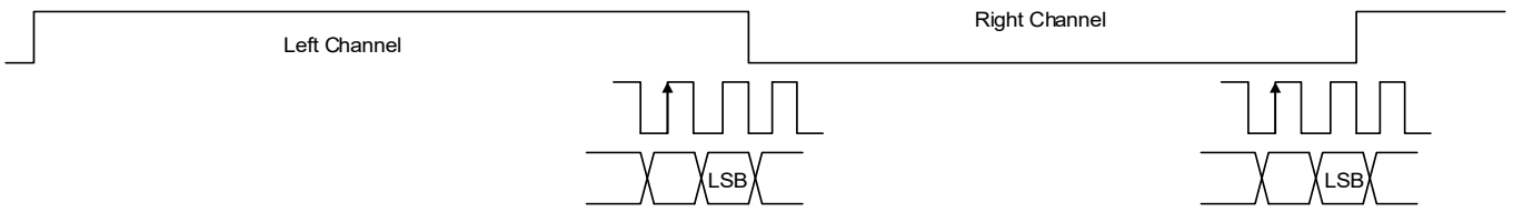
Figure 6. Right-Justified
