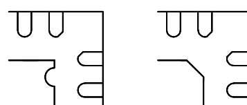
Pin #1 ID and Tie Bar Mark Options
