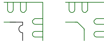
Pin #1 ID and Tie Bar Mark Options
