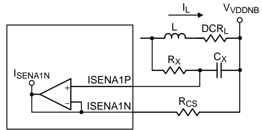
Figure 19. VDDNB Controller : Lossless Inductor Sensing
